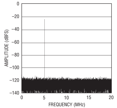
LTC2204: 64K Point FFT, 40Msps, f_{IN} = 5.1\text{MHz} , -25dBFS, PGA = 0, DITH = 1
